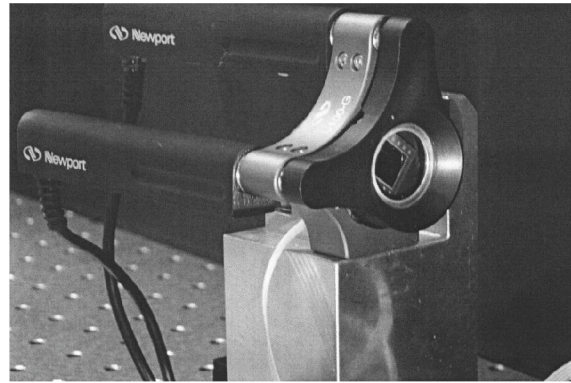
Fig. 2. Ultrafast mirror mounted with motorized positioners in front of the quadrature detector.
