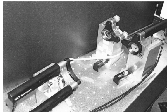
Fig. 3. The BAGLE prototype.
