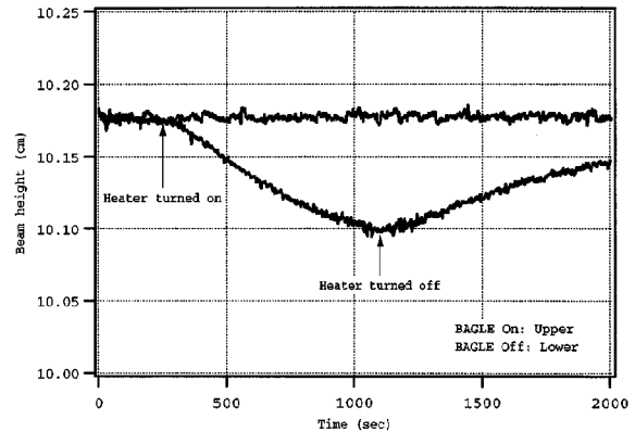
Fig. 8. Measured beam height as a function of time with a space heater set directly underneath the optical table.
