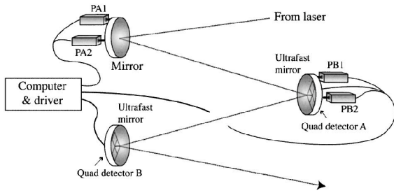
Fig. 1. BAGLE components.
