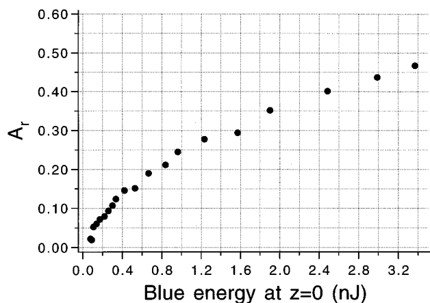
Fig. 6. BLIRA in a \text{LiTaO}_3 waveguide. Here we plot the BLIRA factor A_r [1 minus the red transmitted energy E_r(L, E_{\text{in}}) in the presence of blue light divided by the red transmitted energy E_r(L, 0) without blue light] from Eq. (38) as a function of input blue energy.
