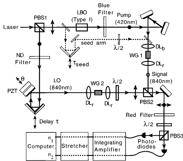
Fig. 2. Schematic of squeezing experiment. The seed arm is used only for study of blue-light-induced red absorption.
