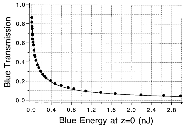
Fig. 5. TPA of blue light in a \text{LiTaO}_3 waveguide. Here we plot the transmission of a blue pulse versus input blue energy.
