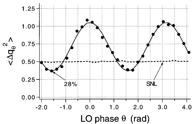
Fig. 3. Squeezed quadrature variance versus LO phase. Filled circles, data; solid curve, fit to Eq. (31) with \eta_{\text{det}}\eta_{\text{temp}} = 0.36 and s_{\text{eff}} = 0.71 ; dashed curve, shot-noise level.
